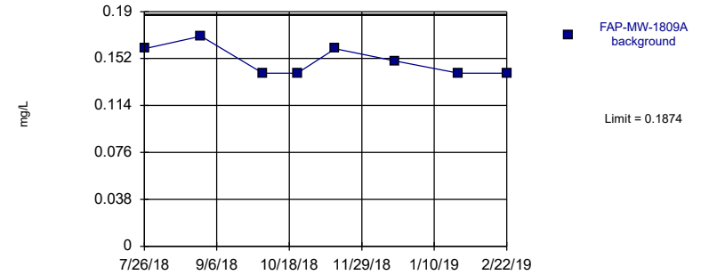
Prediction Limit Intrawell Parametric, FAP-MW-1809A (bg)
