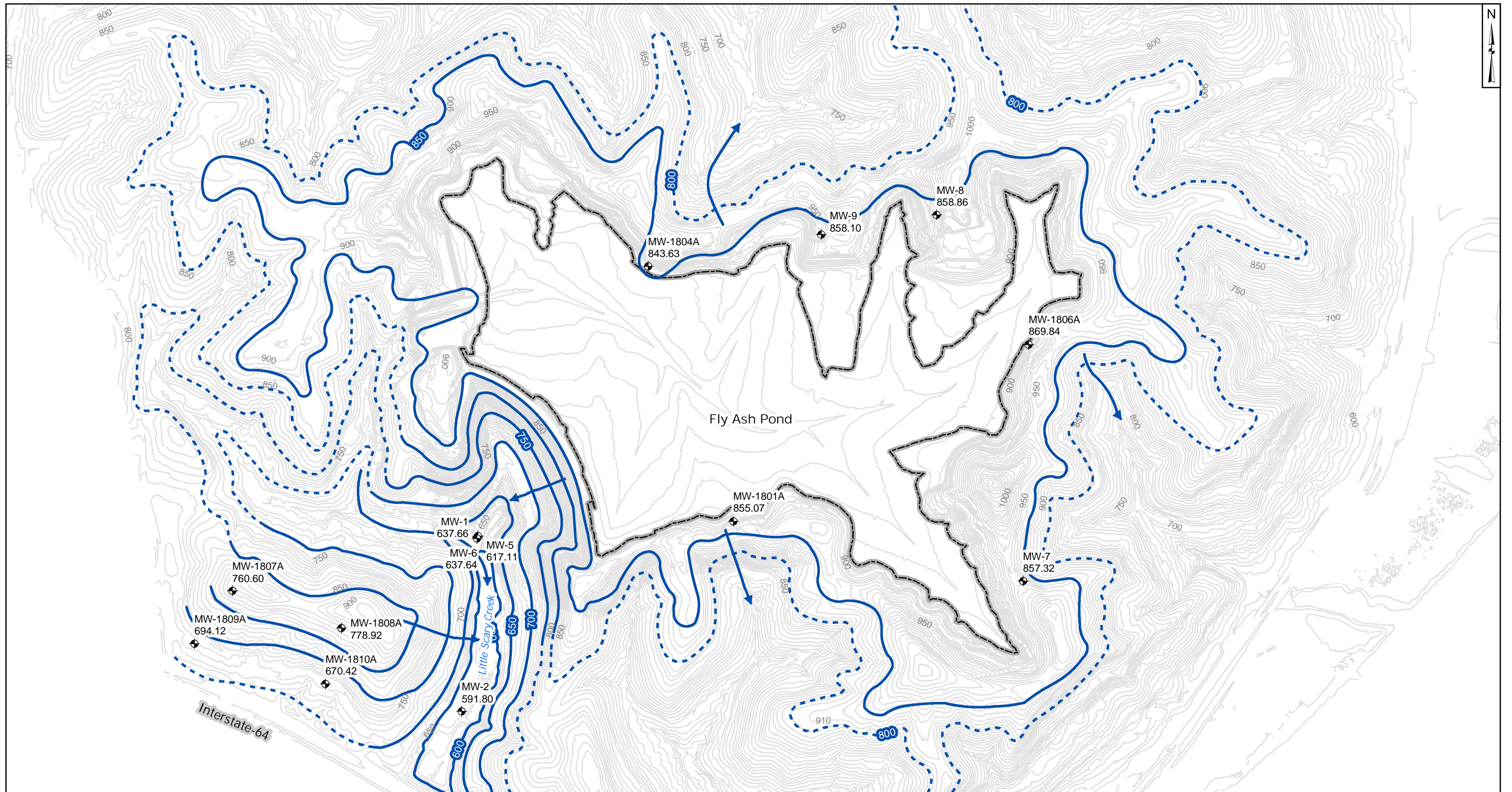
Potentiometric Surface Map - Uppermost Aquifer February 2019
