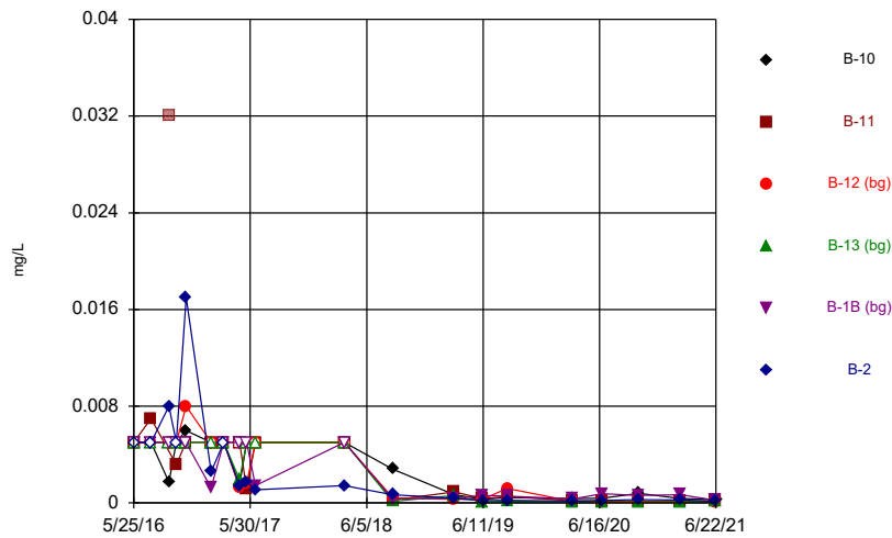
Constituent: Arsenic, total Analysis Run 8/31/2021 12:39 PM Flint Creek Landfill Client: Geosyntec Data: Flint Creek LF
