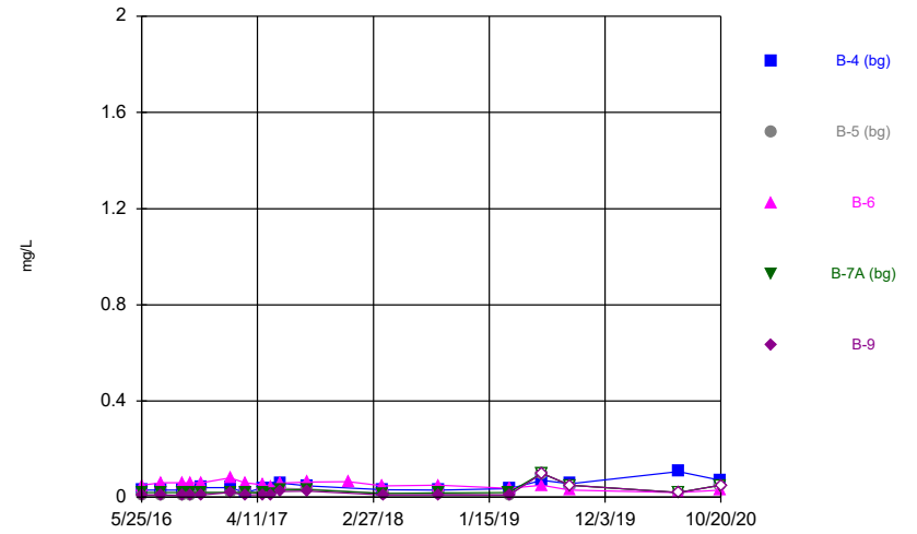
Constituent: Boron, total Analysis Run 2/4/2021 9:47 AM Flint Creek Landfill Client: Geosyntec Data: Flint Creek LF
