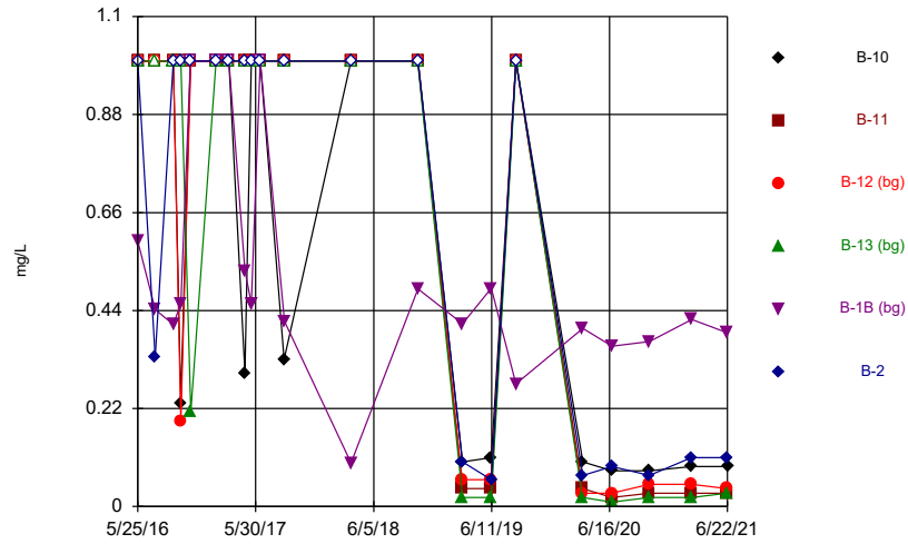
Constituent: Fluoride, total Analysis Run 8/31/2021 12:39 PM Flint Creek Landfill Client: Geosyntec Data: Flint Creek LF
