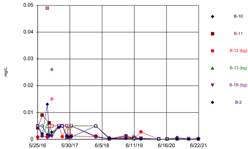
Constituent: Lead, total Analysis Run 8/31/2021 12:39 PM Flint Creek Landfill Client: Geosyntec Data: Flint Creek LF
