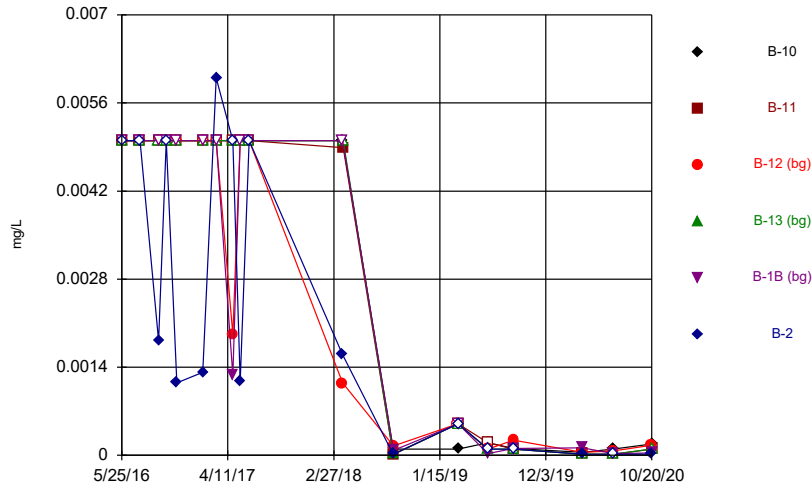
Constituent: Antimony, total Analysis Run 2/4/2021 9:47 AM Flint Creek Landfill Client: Geosyntec Data: Flint Creek LF
