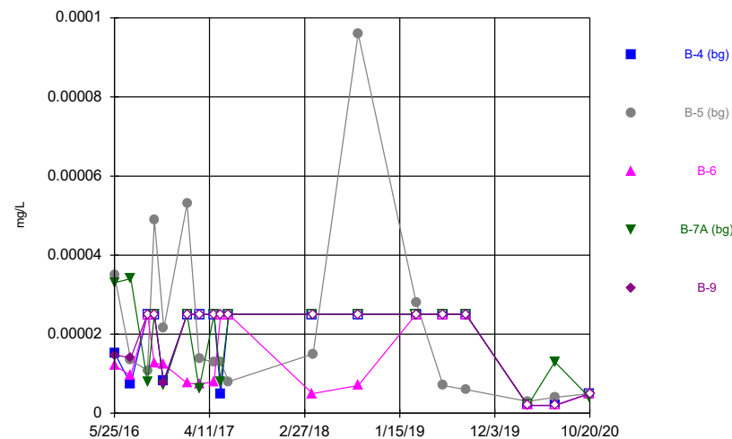
Constituent: Mercury, total Analysis Run 2/4/2021 9:47 AM Flint Creek Landfill Client: Geosyntec Data: Flint Creek LF
