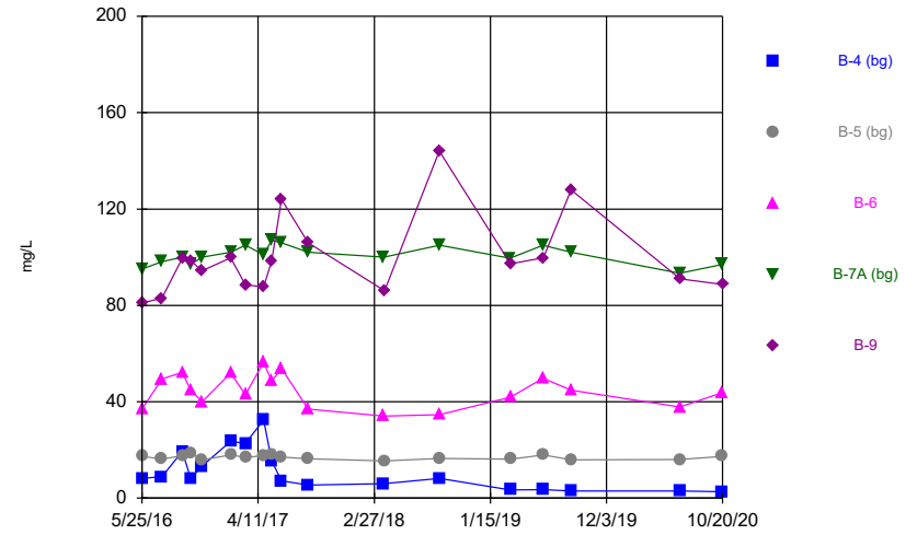
Constituent: Calcium, total Analysis Run 2/4/2021 9:47 AM Flint Creek Landfill Client: Geosyntec Data: Flint Creek LF
