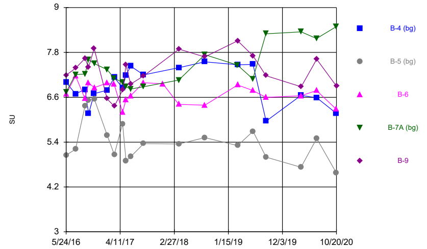
Constituent: pH, field Analysis Run 2/4/2021 9:47 AM Flint Creek Landfill Client: Geosyntec Data: Flint Creek LF
