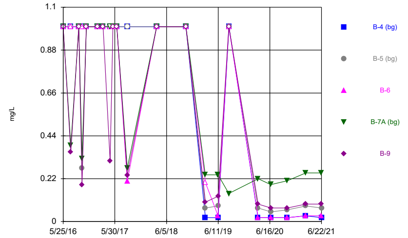
Constituent: Fluoride, total Analysis Run 8/31/2021 12:39 PM Flint Creek Landfill Client: Geosyntec Data: Flint Creek LF
