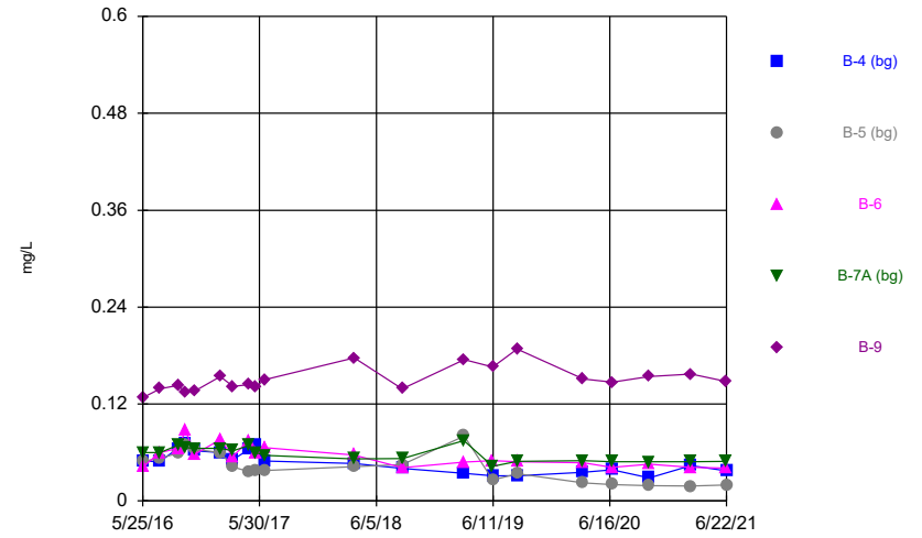
Constituent: Barium, total Analysis Run 8/31/2021 12:39 PM Flint Creek Landfill Client: Geosyntec Data: Flint Creek LF
