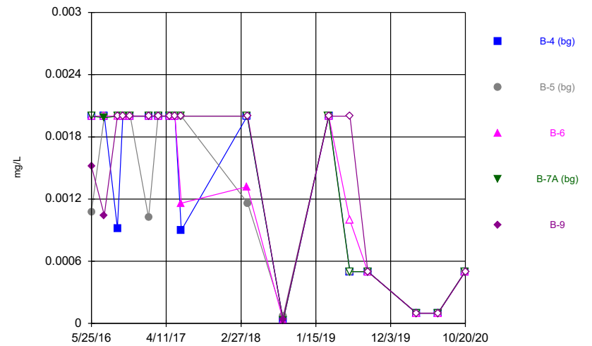
Constituent: Thallium, total Analysis Run 2/4/2021 9:47 AM Flint Creek Landfill Client: Geosyntec Data: Flint Creek LF
