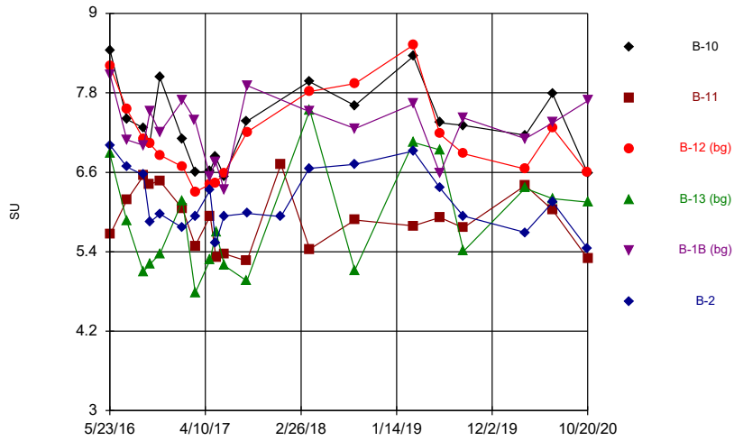
Constituent: pH, field Analysis Run 2/4/2021 9:47 AM Flint Creek Landfill Client: Geosyntec Data: Flint Creek LF
