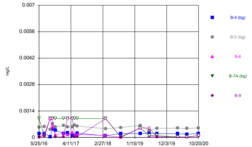
Constituent: Beryllium, total Analysis Run 2/4/2021 9:47 AM Flint Creek Landfill Client: Geosyntec Data: Flint Creek LF
