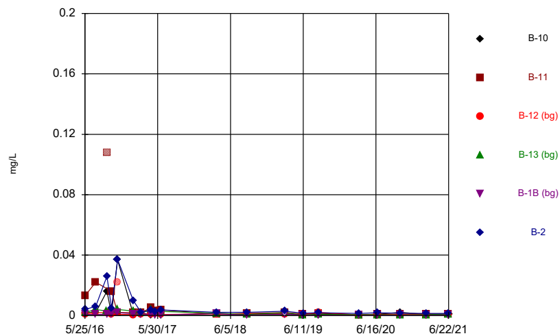
Constituent: Chromium, total Analysis Run 8/31/2021 12:39 PM Flint Creek Landfill Client: Geosyntec Data: Flint Creek LF
