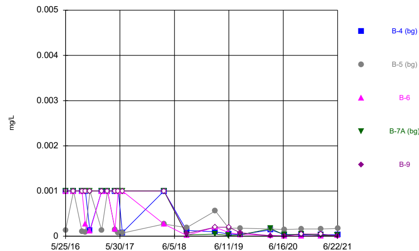
Constituent: Cadmium, total Analysis Run 8/31/2021 12:39 PM Flint Creek Landfill Client: Geosyntec Data: Flint Creek LF
