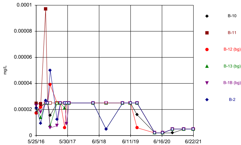
Constituent: Mercury, total Analysis Run 8/31/2021 12:39 PM Flint Creek Landfill Client: Geosyntec Data: Flint Creek LF
