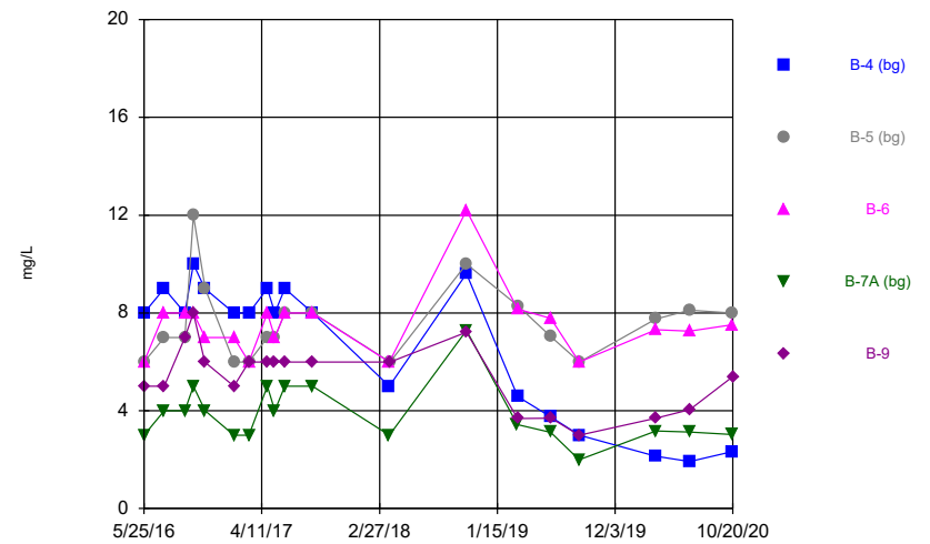
Constituent: Chloride, total Analysis Run 2/4/2021 9:47 AM Flint Creek Landfill Client: Geosyntec Data: Flint Creek LF
