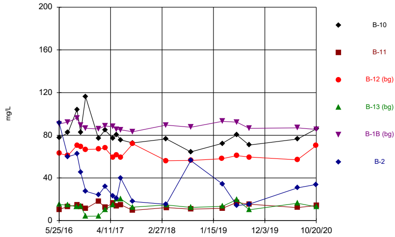
Constituent: Calcium, total Analysis Run 2/4/2021 9:47 AM Flint Creek Landfill Client: Geosyntec Data: Flint Creek LF
