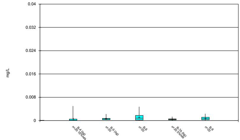
Constituent: Cobalt, total Analysis Run 8/31/2021 12:40 PM Flint Creek Landfill Client: Geosyntec Data: Flint Creek LF
