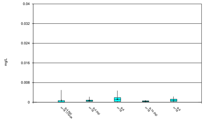
Constituent: Cobalt, total Analysis Run 2/4/2021 9:49 AM Flint Creek Landfill Client: Geosyntec Data: Flint Creek LF
