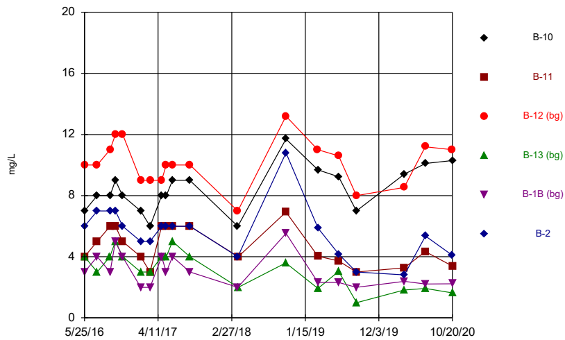
Constituent: Chloride, total Analysis Run 2/4/2021 9:47 AM Flint Creek Landfill Client: Geosyntec Data: Flint Creek LF
