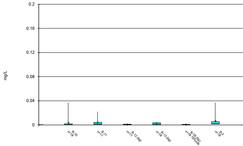
Constituent: Chromium, total Analysis Run 2/4/2021 9:48 AM Flint Creek Landfill Client: Geosyntec Data: Flint Creek LF
