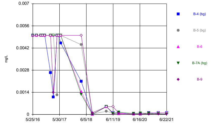
Constituent: Antimony, total Analysis Run 8/31/2021 12:39 PM Flint Creek Landfill Client: Geosyntec Data: Flint Creek LF
