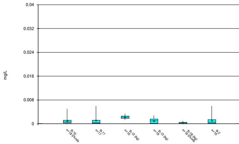
Constituent: Cobalt, total Analysis Run 2/4/2021 9:49 AM Flint Creek Landfill Client: Geosyntec Data: Flint Creek LF
