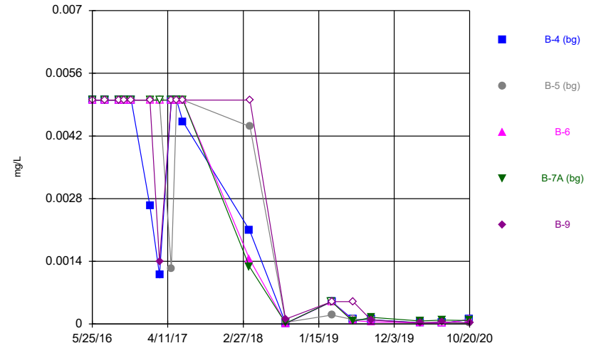
Constituent: Antimony, total Analysis Run 2/4/2021 9:47 AM Flint Creek Landfill Client: Geosyntec Data: Flint Creek LF
