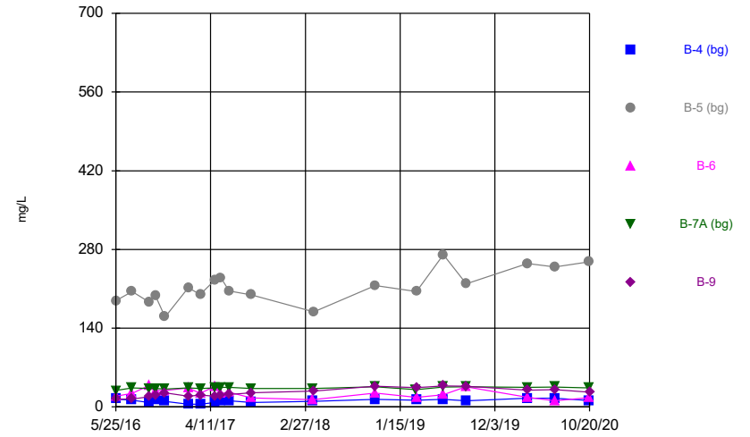
Constituent: Sulfate, total Analysis Run 2/4/2021 9:47 AM Flint Creek Landfill Client: Geosyntec Data: Flint Creek LF
