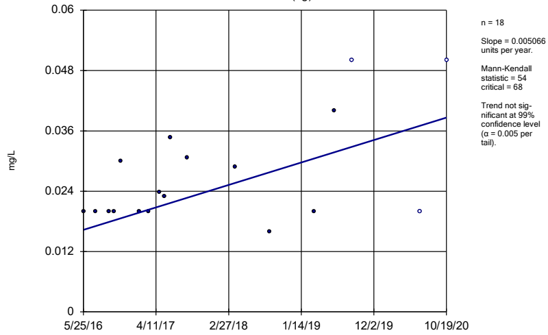
Sen's Slope Estimator B-12 (bg)
