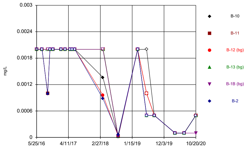
Constituent: Thallium, total Analysis Run 2/4/2021 9:47 AM Flint Creek Landfill Client: Geosyntec Data: Flint Creek LF
