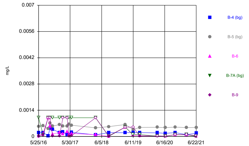
Constituent: Beryllium, total Analysis Run 8/31/2021 12:39 PM Flint Creek Landfill Client: Geosyntec Data: Flint Creek LF
