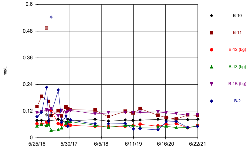
Constituent: Barium, total Analysis Run 8/31/2021 12:39 PM Flint Creek Landfill Client: Geosyntec Data: Flint Creek LF
