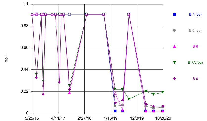
Constituent: Fluoride, total Analysis Run 2/4/2021 9:47 AM Flint Creek Landfill Client: Geosyntec Data: Flint Creek LF
