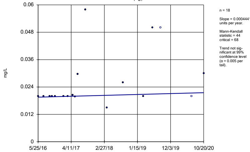
Sen's Slope Estimator B-1B (bg)
