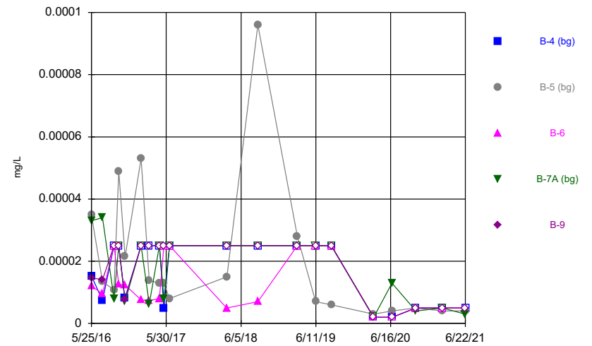
Constituent: Mercury, total Analysis Run 8/31/2021 12:39 PM Flint Creek Landfill Client: Geosyntec Data: Flint Creek LF
