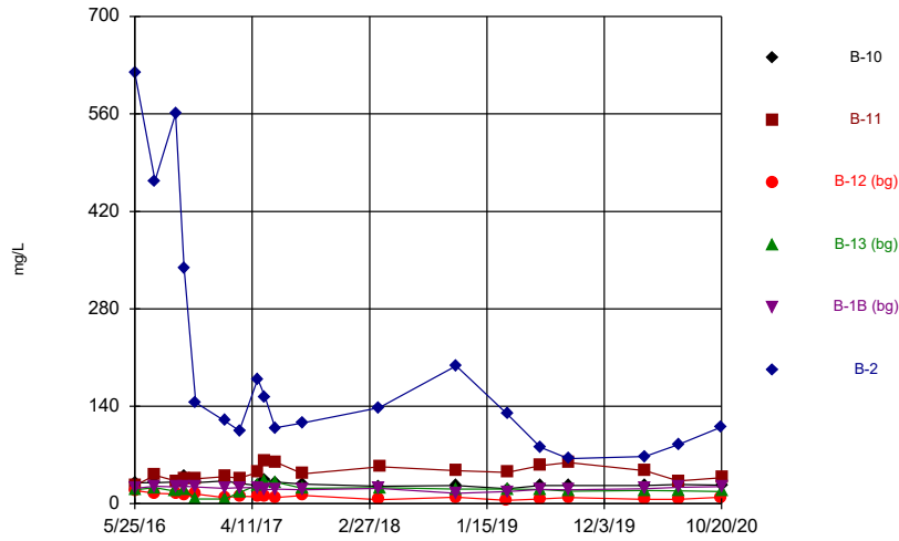
Constituent: Sulfate, total Analysis Run 2/4/2021 9:47 AM Flint Creek Landfill Client: Geosyntec Data: Flint Creek LF
