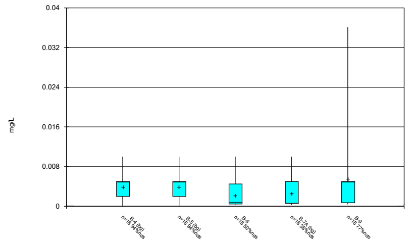
Constituent: Molybdenum, total Analysis Run 2/4/2021 9:49 AM Flint Creek Landfill Client: Geosyntec Data: Flint Creek LF
