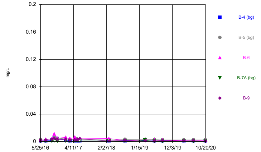
Constituent: Chromium, total Analysis Run 2/4/2021 9:47 AM Flint Creek Landfill Client: Geosyntec Data: Flint Creek LF
