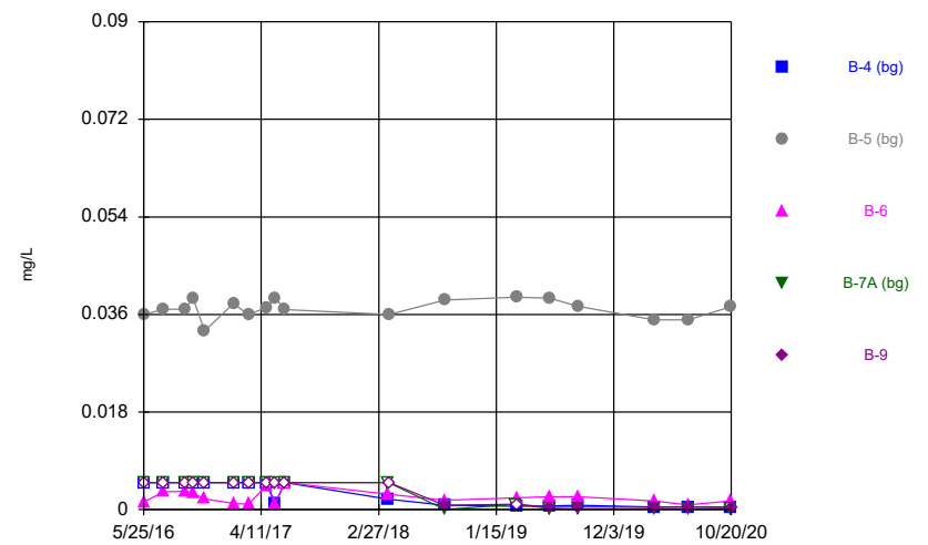
Constituent: Selenium, total Analysis Run 2/4/2021 9:47 AM Flint Creek Landfill Client: Geosyntec Data: Flint Creek LF
