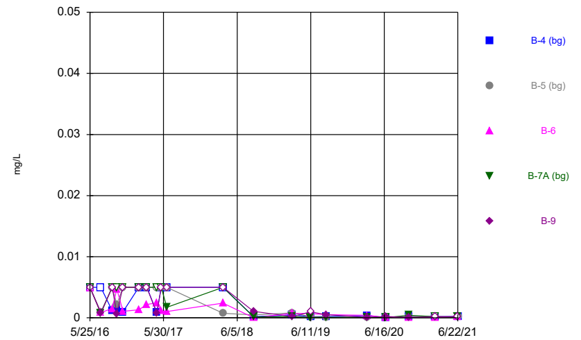
Constituent: Lead, total Analysis Run 8/31/2021 12:39 PM Flint Creek Landfill Client: Geosyntec Data: Flint Creek LF
