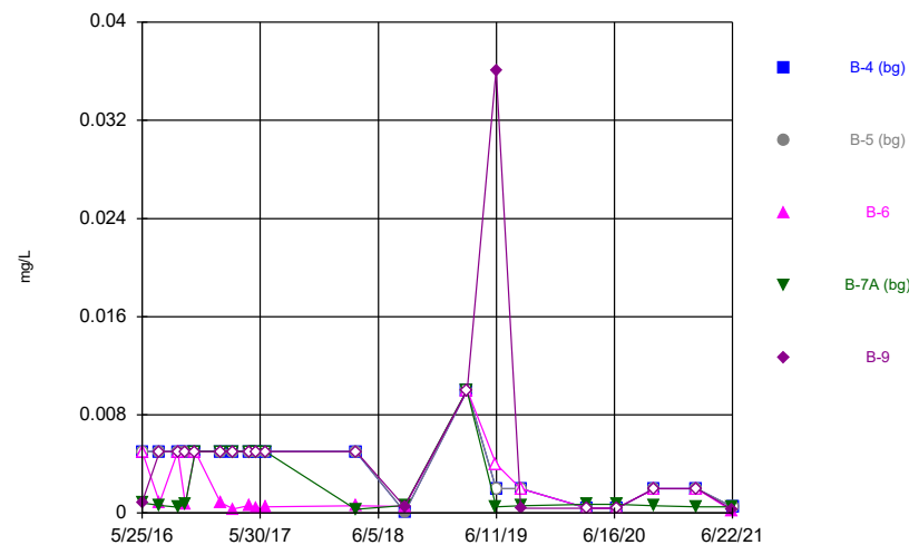
Constituent: Molybdenum, total Analysis Run 8/31/2021 12:39 PM Flint Creek Landfill Client: Geosyntec Data: Flint Creek LF
