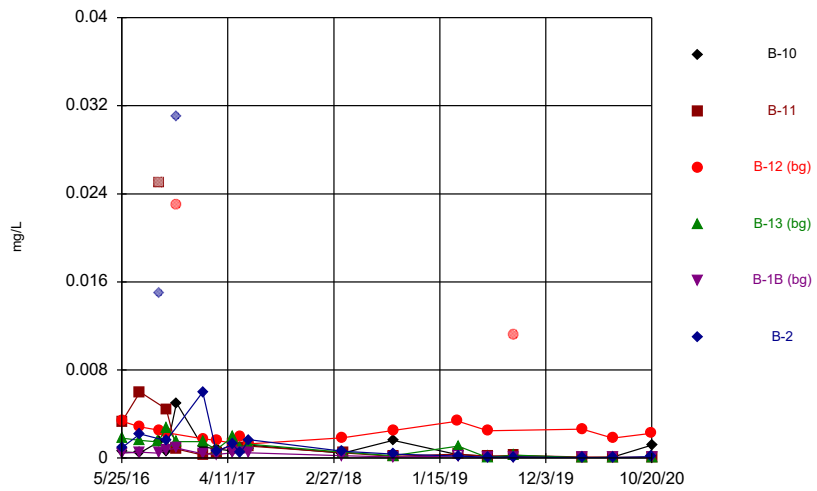
Constituent: Cobalt, total Analysis Run 2/4/2021 9:47 AM Flint Creek Landfill Client: Geosyntec Data: Flint Creek LF
