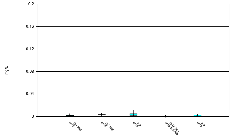
Constituent: Chromium, total Analysis Run 2/4/2021 9:49 AM Flint Creek Landfill Client: Geosyntec Data: Flint Creek LF
