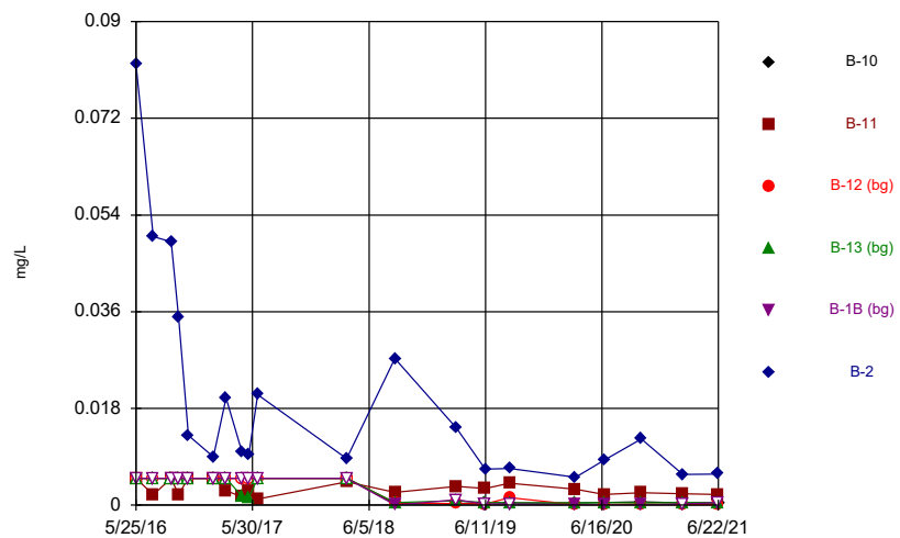
Constituent: Selenium, total Analysis Run 8/31/2021 12:39 PM Flint Creek Landfill Client: Geosyntec Data: Flint Creek LF
