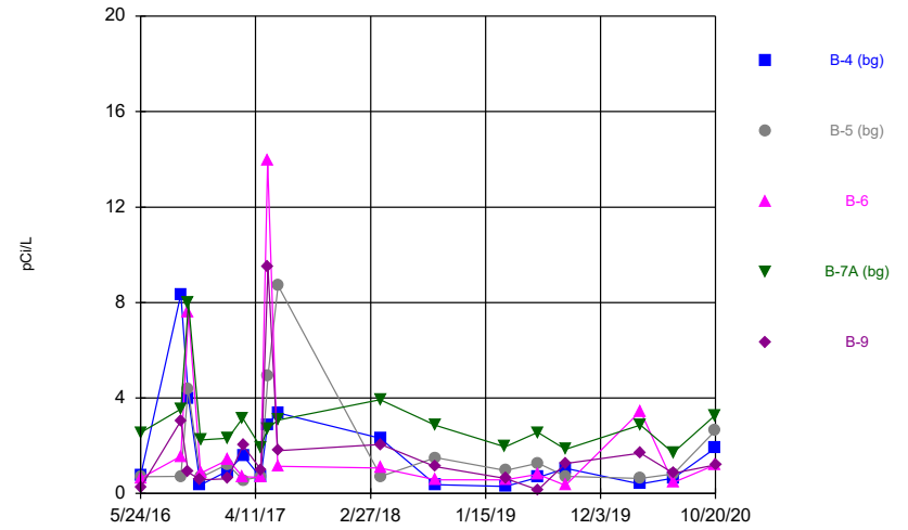
Constituent: Combined Radium 226 + 228 Analysis Run 2/4/2021 9:47 AM Flint Creek Landfill Client: Geosyntec Data: Flint Creek LF
