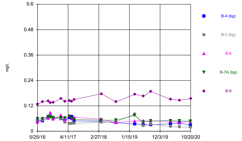
Constituent: Barium, total Analysis Run 2/4/2021 9:47 AM Flint Creek Landfill Client: Geosyntec Data: Flint Creek LF
