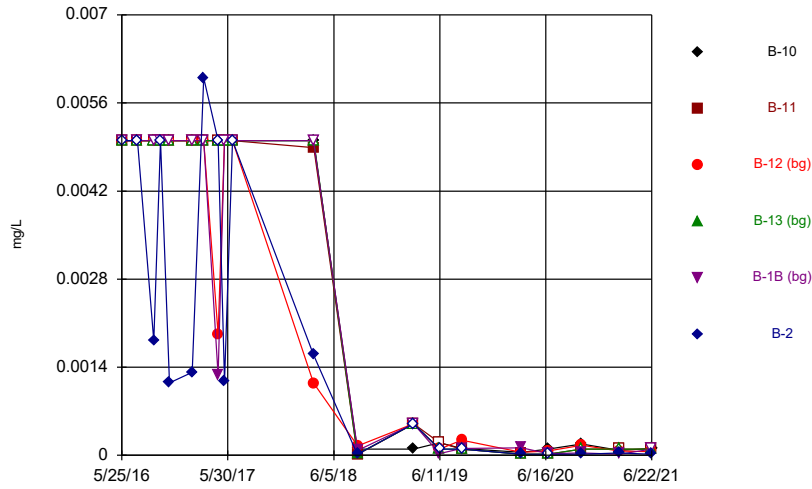
Constituent: Antimony, total Analysis Run 8/31/2021 12:39 PM Flint Creek Landfill Client: Geosyntec Data: Flint Creek LF
