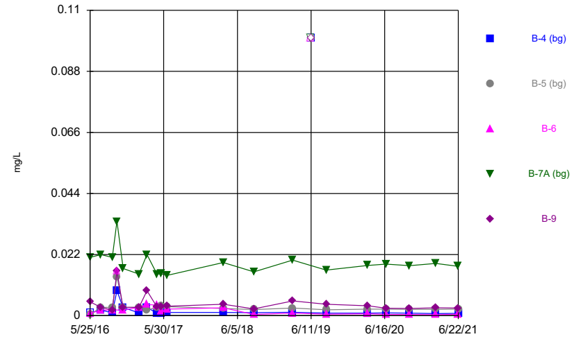
Constituent: Lithium, total Analysis Run 8/31/2021 12:39 PM Flint Creek Landfill Client: Geosyntec Data: Flint Creek LF
