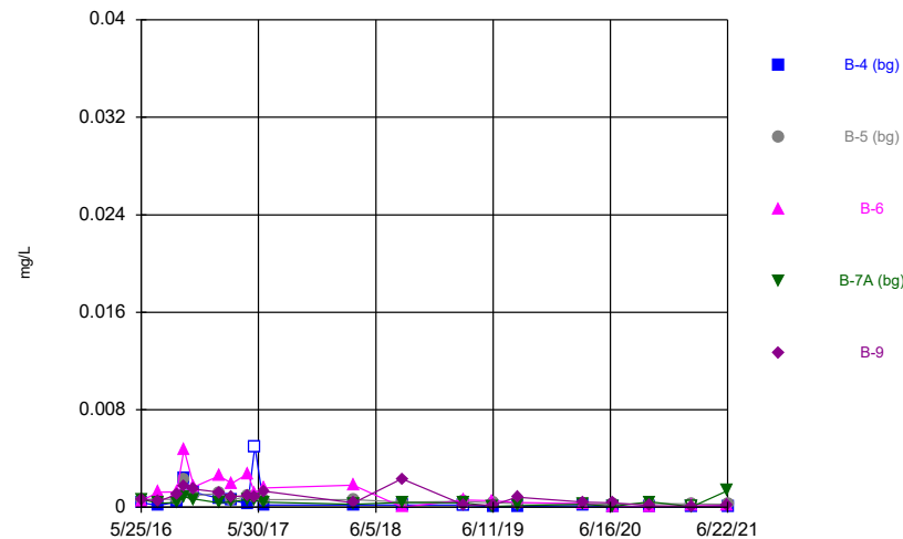
Constituent: Cobalt, total Analysis Run 8/31/2021 12:39 PM Flint Creek Landfill Client: Geosyntec Data: Flint Creek LF
