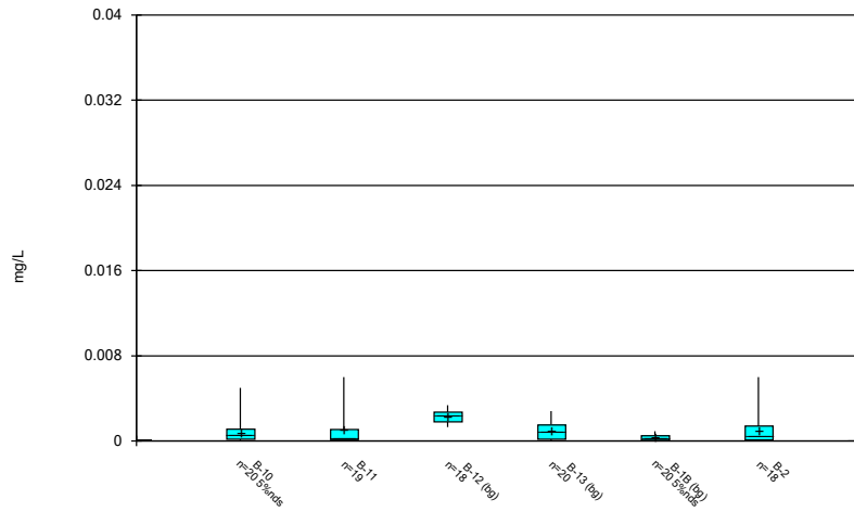
Constituent: Cobalt, total Analysis Run 8/31/2021 12:40 PM Flint Creek Landfill Client: Geosyntec Data: Flint Creek LF
