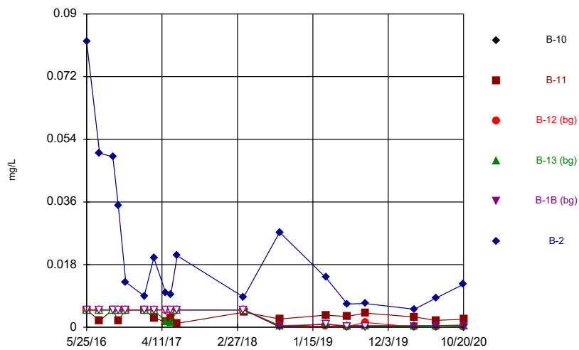
Constituent: Selenium, total Analysis Run 2/4/2021 9:47 AM Flint Creek Landfill Client: Geosyntec Data: Flint Creek LF
