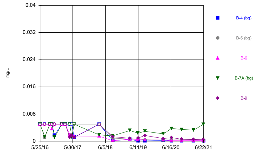
Constituent: Arsenic, total Analysis Run 8/31/2021 12:39 PM Flint Creek Landfill Client: Geosyntec Data: Flint Creek LF
