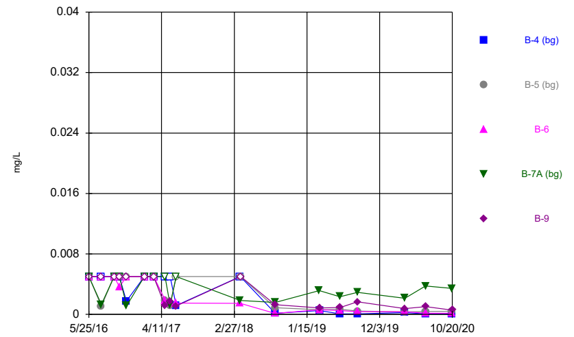
Constituent: Arsenic, total Analysis Run 2/4/2021 9:47 AM Flint Creek Landfill Client: Geosyntec Data: Flint Creek LF
