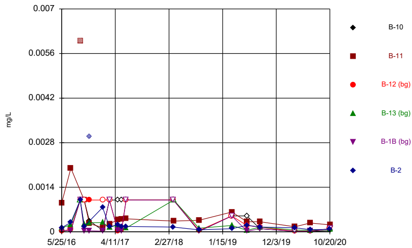
Constituent: Beryllium, total Analysis Run 2/4/2021 9:47 AM Flint Creek Landfill Client: Geosyntec Data: Flint Creek LF
