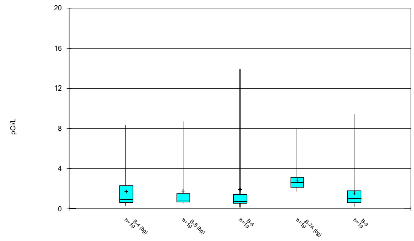
Constituent: Combined Radium 226 + 228 Analysis Run 8/31/2021 12:40 PM Flint Creek Landfill Client: Geosyntec Data: Flint Creek LF
