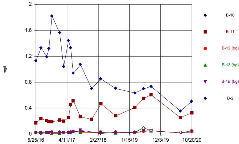
Constituent: Boron, total Analysis Run 2/4/2021 9:47 AM Flint Creek Landfill Client: Geosyntec Data: Flint Creek LF
