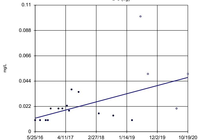
Sen's Slope Estimator B-5 (bg)
