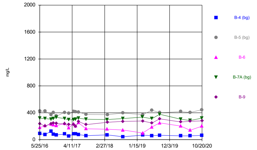
Constituent: Total Dissolved Solids [TDS] Analysis Run 2/4/2021 9:47 AM Flint Creek Landfill Client: Geosyntec Data: Flint Creek LF
