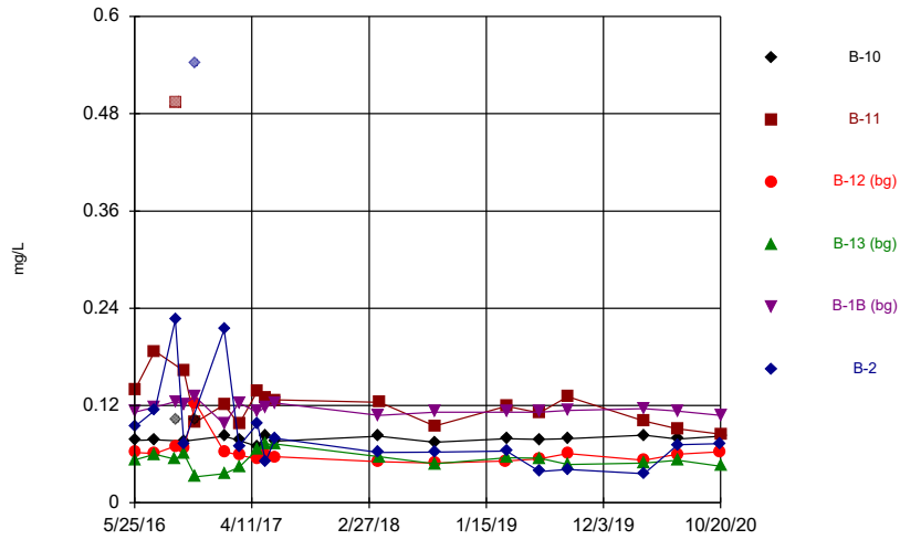
Constituent: Barium, total Analysis Run 2/4/2021 9:47 AM Flint Creek Landfill Client: Geosyntec Data: Flint Creek LF
