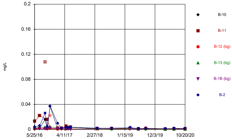
Constituent: Chromium, total Analysis Run 2/4/2021 9:47 AM Flint Creek Landfill Client: Geosyntec Data: Flint Creek LF
