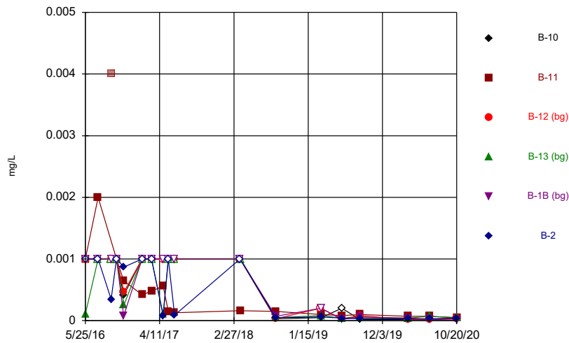
Constituent: Cadmium, total Analysis Run 2/4/2021 9:47 AM Flint Creek Landfill Client: Geosyntec Data: Flint Creek LF
