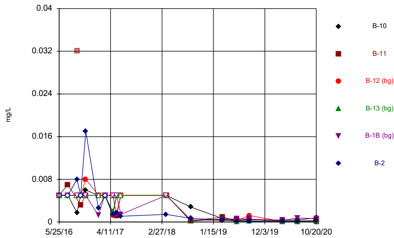
Constituent: Arsenic, total Analysis Run 2/4/2021 9:47 AM Flint Creek Landfill Client: Geosyntec Data: Flint Creek LF
