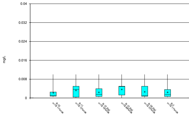
Constituent: Molybdenum, total Analysis Run 2/4/2021 9:49 AM Flint Creek Landfill Client: Geosyntec Data: Flint Creek LF
