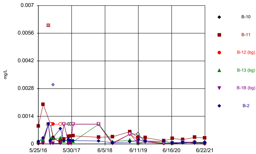
Constituent: Beryllium, total Analysis Run 8/31/2021 12:39 PM Flint Creek Landfill Client: Geosyntec Data: Flint Creek LF
