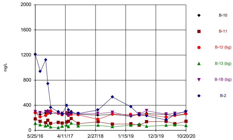
Constituent: Total Dissolved Solids [TDS] Analysis Run 2/4/2021 9:47 AM Flint Creek Landfill Client: Geosyntec Data: Flint Creek LF
