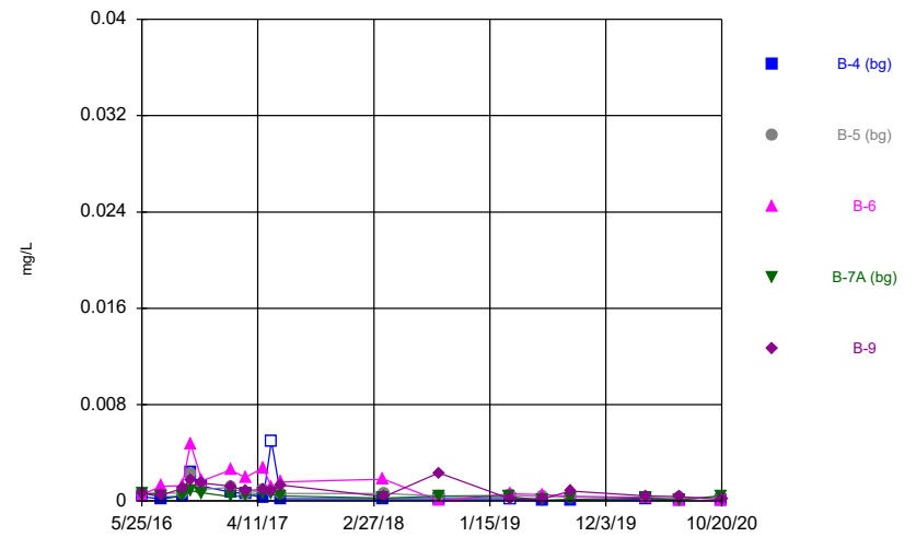
Constituent: Cobalt, total Analysis Run 2/4/2021 9:47 AM Flint Creek Landfill Client: Geosyntec Data: Flint Creek LF
