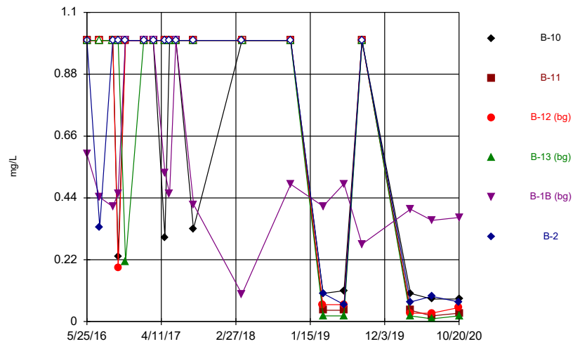
Constituent: Fluoride, total Analysis Run 2/4/2021 9:47 AM Flint Creek Landfill Client: Geosyntec Data: Flint Creek LF
