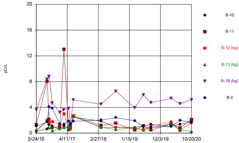
Constituent: Combined Radium 226 + 228 Analysis Run 2/4/2021 9:47 AM Flint Creek Landfill Client: Geosyntec Data: Flint Creek LF
