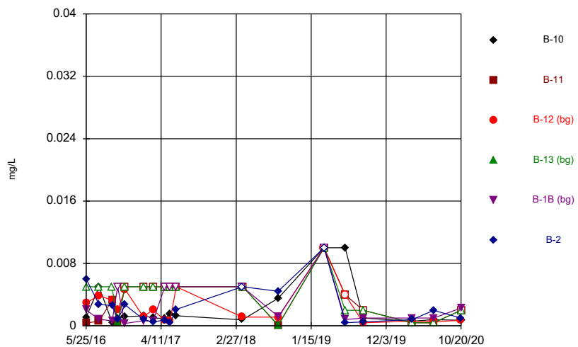
Constituent: Molybdenum, total Analysis Run 2/4/2021 9:47 AM Flint Creek Landfill Client: Geosyntec Data: Flint Creek LF
