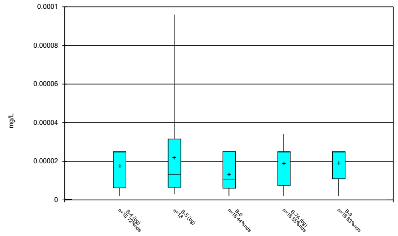
Constituent: Mercury, total Analysis Run 2/4/2021 9:49 AM Flint Creek Landfill Client: Geosyntec Data: Flint Creek LF
