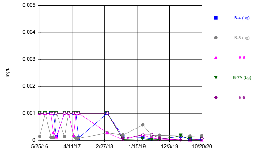
Constituent: Cadmium, total Analysis Run 2/4/2021 9:47 AM Flint Creek Landfill Client: Geosyntec Data: Flint Creek LF
