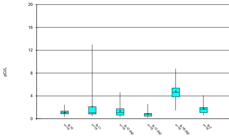
Constituent: Combined Radium 226 + 228 Analysis Run 8/31/2021 12:40 PM Flint Creek Landfill Client: Geosyntec Data: Flint Creek LF
