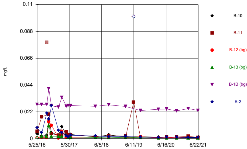
Constituent: Lithium, total Analysis Run 8/31/2021 12:39 PM Flint Creek Landfill Client: Geosyntec Data: Flint Creek LF
