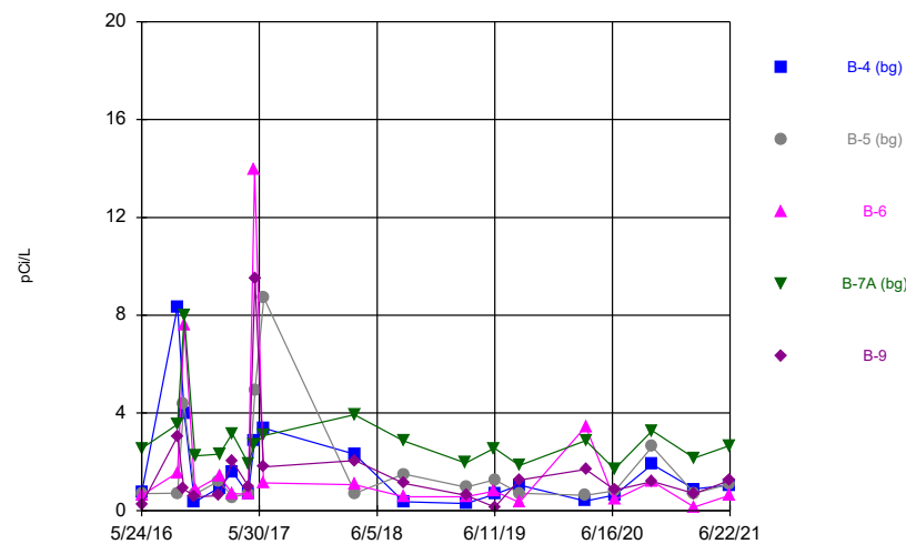
Constituent: Combined Radium 226 + 228 Analysis Run 8/31/2021 12:39 PM Flint Creek Landfill Client: Geosyntec Data: Flint Creek LF
